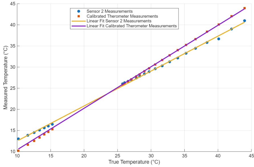
Figure 5.2: Sensor two vs calibrated sensor
